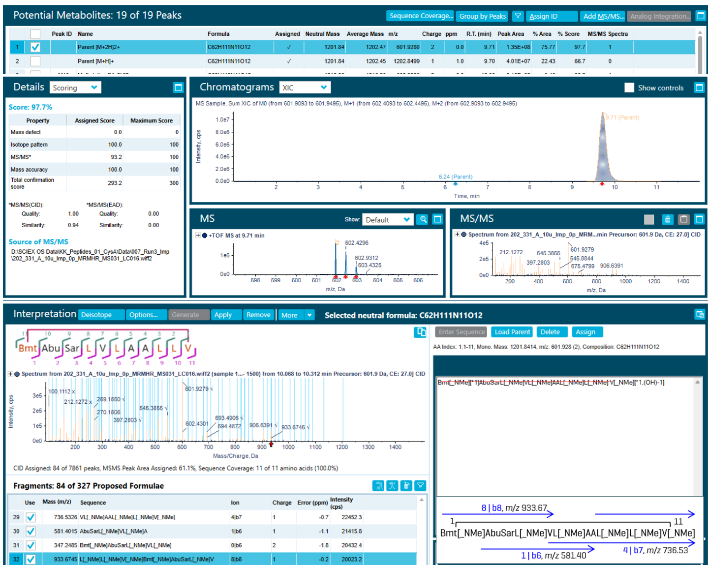
Figure 6. Results [top] and fragment interpretation (bottom) of CysA. The result view shows chromatograms, MS, and CID-MS/MS and the interpretation view allows sequence analysis using CID-MS/MS. Common product ion peaks matched to the selected parent MS/MS spectrum in the processing parameters are shown in orange. Blue lines indicate peaks assigned to the sequence. The fragment ions are assigned as cyclic structures (bottom right). Annotation details are shown in Figure 8.
