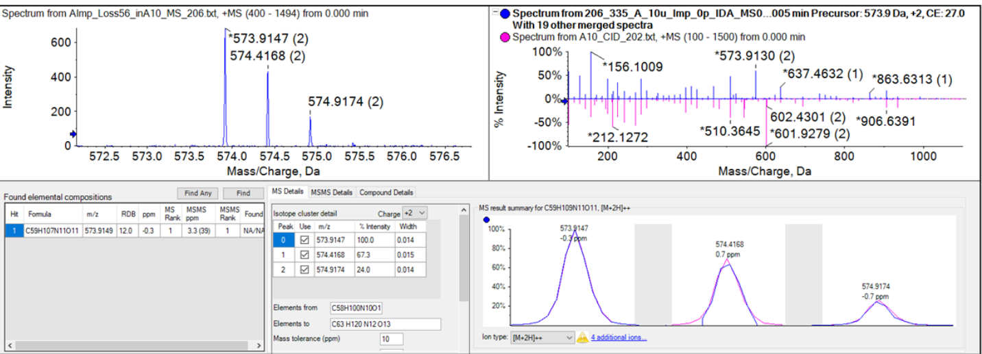
Figure 12. Formula prediction using formula finder in SCIEX OS software. Molecular formula of G7 was predicted as C59H107N11O11 (minus C3H4O from CysA using the accurate mass), isotope pattern and MS/MS.
